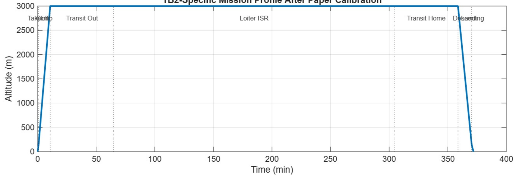
TB2-Specific Mission Profile After Paper Calibration
