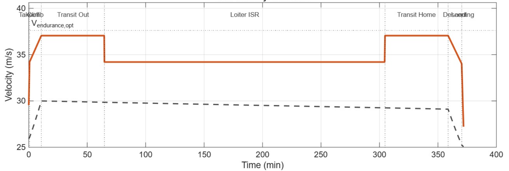
TB2 Velocity Schedule
